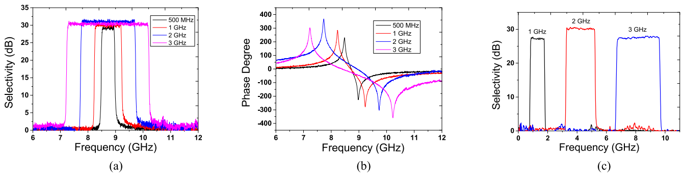
Fig. 6. Filter bandwidth and central frequency tuning and the corresponding phase response.
